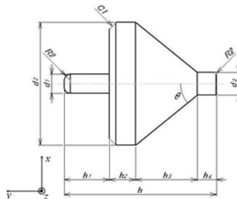
Figure 4-1. Reference shape of spinning tops that do not fall over
