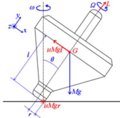
Figure 3-1. Principle of forces acting on spinning top
